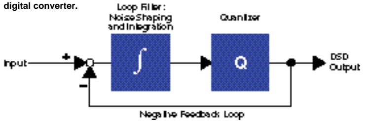
The DSD analog-to-digital converter.
